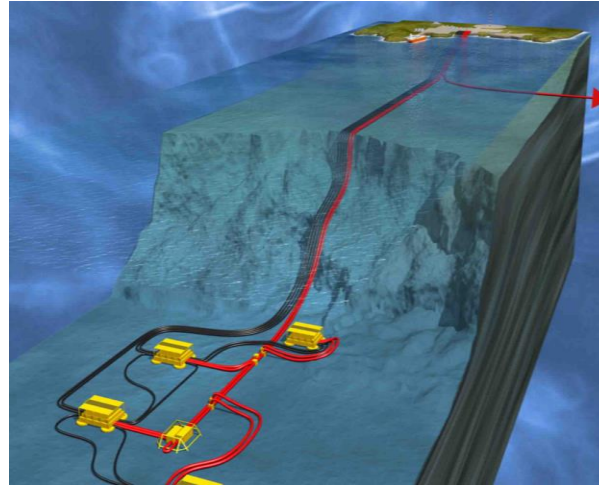
Illustration: Ormen Lange gas field
